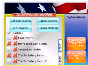
VBS Programming
